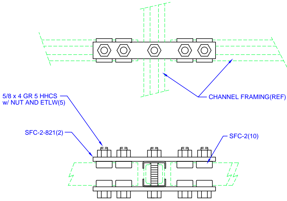
CHANNEL FRAMING SPLICE AT SAME LEVEL (CROSS) GR-1275-CORE
