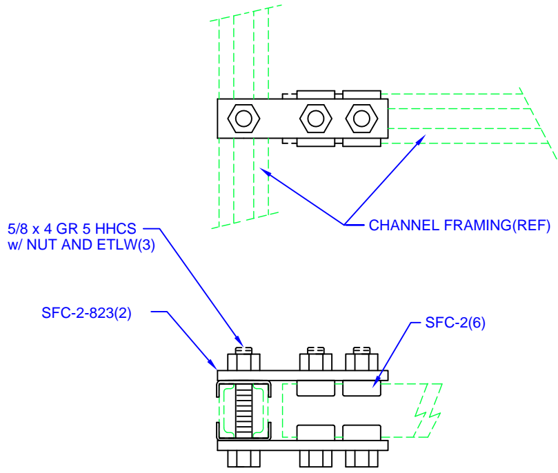
CHANNEL FRAMING SPLICE AT SAME LEVEL (CROSS) GR-1275-CORE
