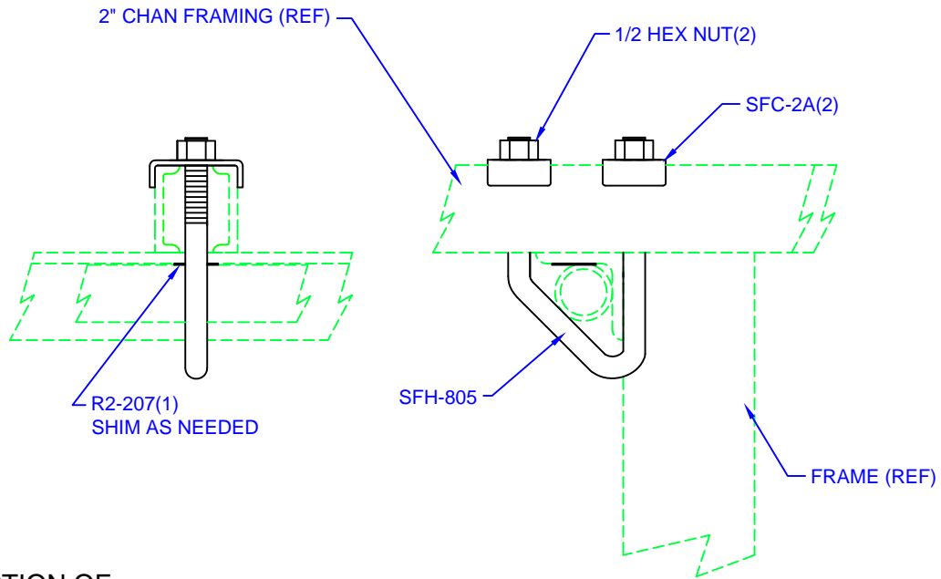
CONNECTION OF: FRAMEWORK ANGLE TO 2" CHANNEL FRAMING.
