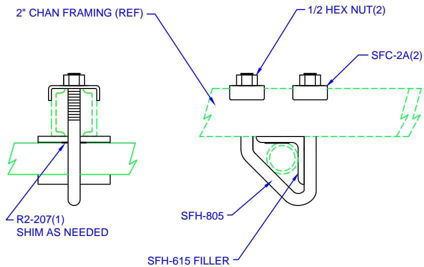
CONNECTION OF: SUPPORT PIPE TO 2" CHANNEL FRAMING(FUTURE FRAME LOCATION)
